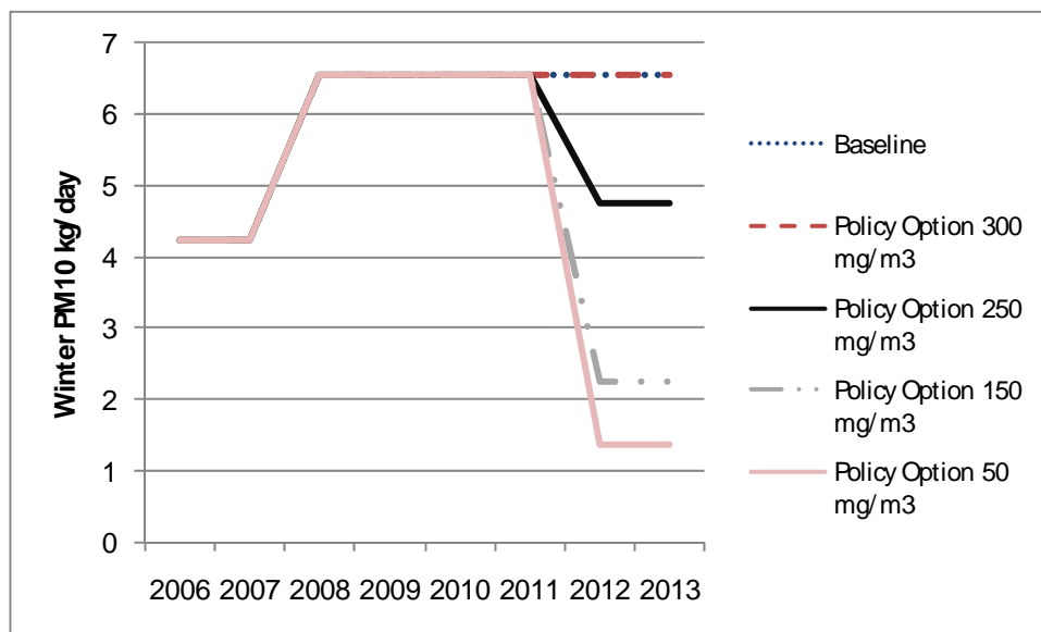
Figure 5.1: Daily PM 10 from coal-fired boilers in Kaiapoi from 2006 to 2013
